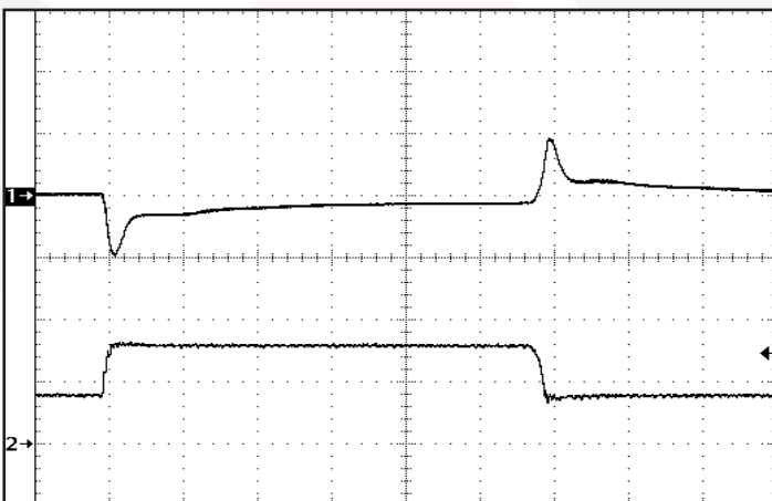
Figure 11: Output voltage response to step-change in load current (50%-100%-50% of Iout(max)). Load cap: 1μF ceramic cap and 10μF, 100 mΩ ESR tantalum cap. Ch 1: Vout (300mV/div). Ch 2: Iout (5A/div).
