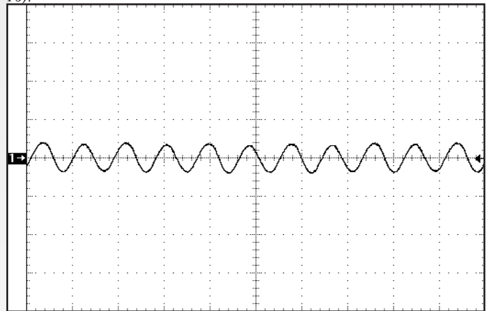
Figure 16: Output voltage ripple, V_{out} , at nominal input voltage and rated load current (10mV/div). Load capacitance: 1µf ceramic capacitor and 10µF tantalum capacitor. Bandwidth: 10 MHz. See Figure 14.
