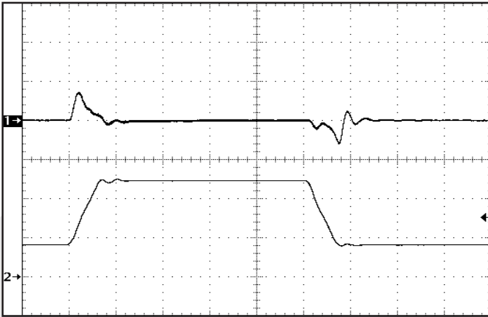
Figure 13: Output voltage response to step-change in input voltage (16V-50V-16V). Load cap 10µF, 100 mΩ ESR tantalum and 1µF ceramic cap. Ch 1: Vout (200mV/div). Ch 2: Vin (20V/div).
